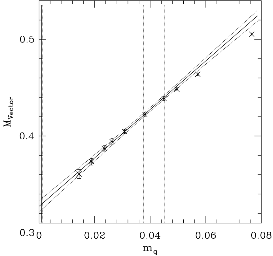
Fig. 25. Plot of M_{\text{vector}} versus the quark mass m . The data, reproduced from [156], were obtained on 32^3 \times 64 quenched lattices at \beta \equiv 6/g^2 = 6 corresponding to 1/a = 2.33(4) GeV. The linear fit is to the lightest six points. The vertical lines show \overline{m} and the range of estimates of m_s .
